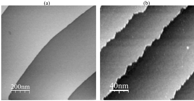
FIG. 1. STM topography of (a) clean iron whisker after repeated cycles of \text{Ar}^+ bombardment and annealing and (b) \text{Fe}(001)\text{-}p(1 \times 1)\text{O} surface. Measurement parameters were I=0.3 nA and U_{\text{gap}}=0.5 V.
