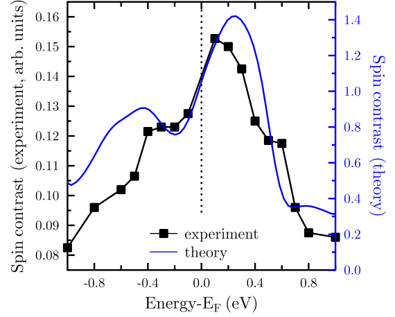
FIG. 4. (Color online) Spin contrast of Fe(001)- p(1 \times 1) O surface: measured as a function of bias voltage from atomically resolved spin-polarized STM (black line) and calculated as a function of energy from the local density of state at 4 Å above the surface layer reflecting the STM experiment (blue line).
