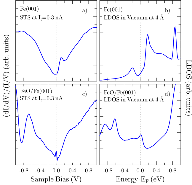
FIG. 3. (Color online) Normalized differential conductance spectra and corresponding spin averaged LDOS calculated at 4 Å above the surface for the clean [(a) and (b)] Fe(001) and [(c) and (d)] Fe(001)- p(1 \times 1) O, respectively. The tip was held at 0.9 V and 0.3 nA, while the voltage was ramped between -0.9 and 0.9 V.
