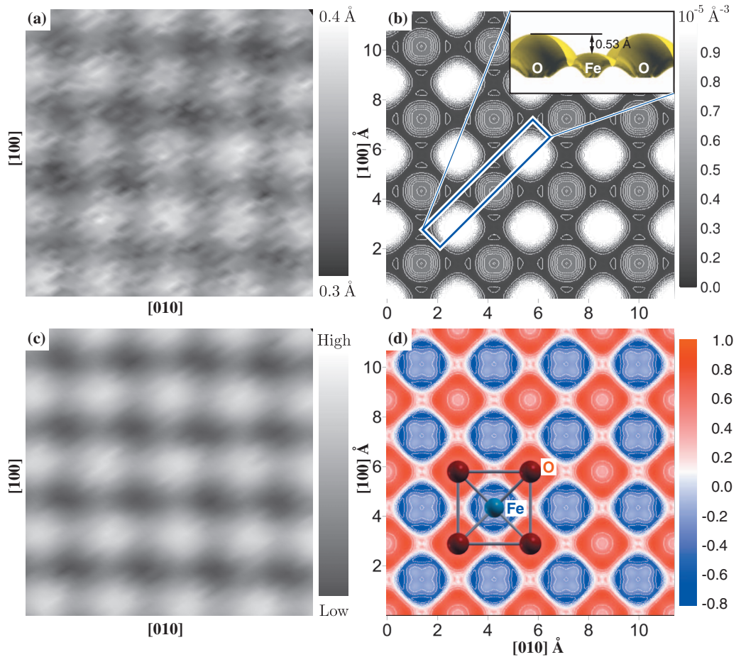
FIG. 2. (Color) (a) Atomically resolved topography of the Fe(001)- p(1 \times 1) O surface. (b) Charge density at the Fermi level calculated in vacuum about 4 Å above the surface [top view of (001) plane]. Inset: equal-density contour of the charge density of 7 \times 10^{-5} \text{ e}\text{\AA}^{-3} calculated on the vertical (110) plane. (c) Spin image obtained simultaneously with the topography in (a) at 0.3 V sample bias. (d) Spin polarization at the Fermi level corresponding to the charge density presented in (b).
