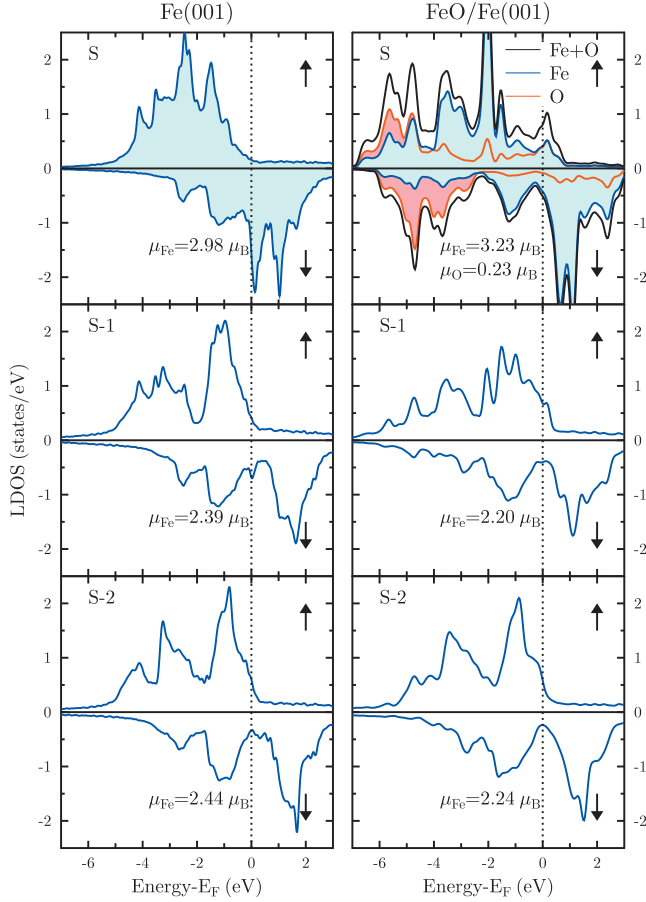
FIG. 5. (Color) Spin resolved densities of states of the surface (s) and two subsurface (S-1, S-2) layers for the clean Fe(001) (left) and Fe(001)- p(1 \times 1)\text{O} (right). Top: black line represents total LDOS of the surface; blue line and shaded area represent the Fe LDOS; red line and shaded area represent the O LDOS.
