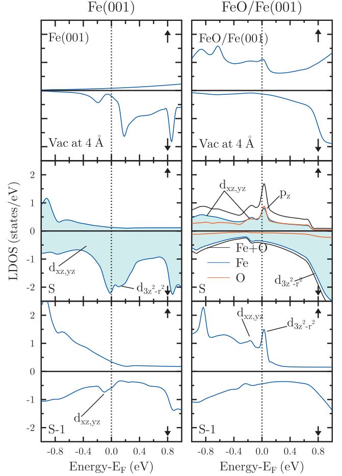
FIG. 6. (Color) Spin resolved densities of states of the vacuum (Vac), surface (s) and subsurface (S-1) layers for the clean Fe(001) (left) and Fe(001)- p(1 \times 1)\text{O} (right) within the energy range corresponding to the applied bias voltage. Only selected states, which participate in the tunneling process, are indicated. Middle (right): black line represents total LDOS of the surface; blue line and shaded area represent the Fe LDOS; red line and shaded area represent the oxygen LDOS.
