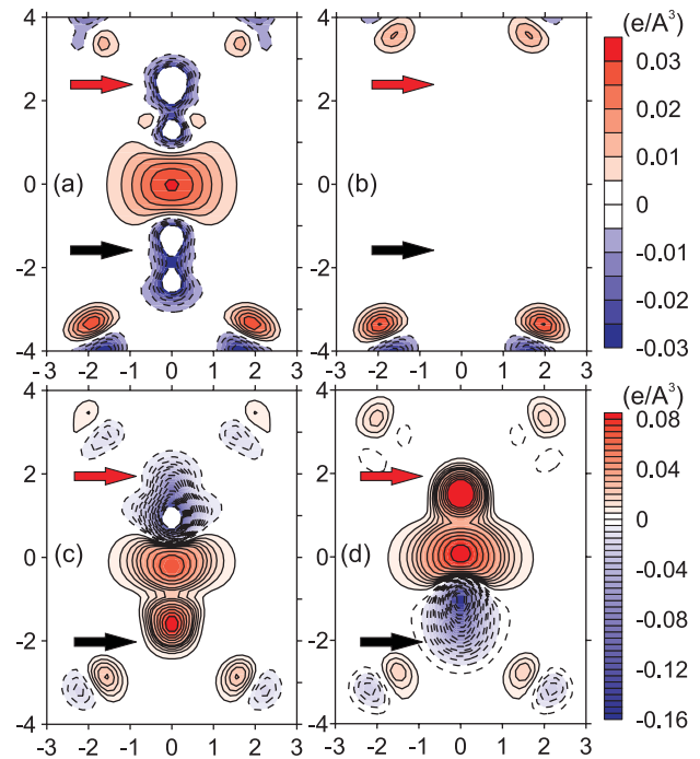
FIG. 2 (color). Spin-dependent charge density difference \Delta\rho^{\sigma} . The red and black arrows in the figure are the positions of the tip apex and the adatom, respectively. The units of the x and y axes are Å. (a) and (b) are the charge density difference for the spin-up and spin-down electrons at the tip-adatom separation of 4.0 Å (P configuration), respectively. (c) and (d) are the charge densities difference for the spin-up and spin-down electrons at the tip-adatom separation of 2.5 Å (AP configuration), respectively.
