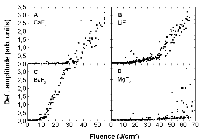
Fig. 3. Fluence dependence of the photoacoustic signal amplitude for different fluoride crystals polished by diamond turning
