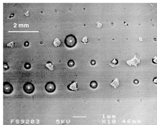
Fig. 5. SEM overview image of damage topographies of diamond turned \text{CaF}_2 (111) surface irradiated with the fluences in range from 18.3 to 55.3 \text{ J/cm}^2 . White spots represent surface damage, dark halos originate from recondensed plasma debris
