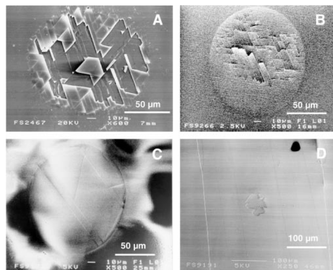
Fig. 2a–d. SEM images of damage topographies of \text{CaF}_2(111) surfaces irradiated with the following fluences: a 27.6 \text{ J/cm}^2 at the conventional standard polish; b 30 \text{ J/cm}^2 at the diamond turned surface; c 57.7 \text{ J/cm}^2 at the chemo-mechanically polished surface; d 46 \text{ J/cm}^2 at the terrace area of a cleaved surface
