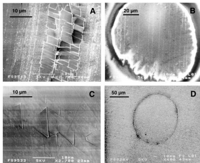
Fig. 4a–d. SEM images of damage topographies of fluoride surfaces polished by diamond turning and irradiated with the following fluences: a \text{CaF}_2 – 36 \text{ J/cm}^2 ; b \text{LiF} – 50.4 \text{ J/cm}^2 ; c \text{BaF}_2 – 12.6 \text{ J/cm}^2 ; d \text{MgF}_2 – 54 \text{ J/cm}^2 . The laser spot diameter is 100 \mu\text{m} in all cases. Notice the magnified scale in a and c
