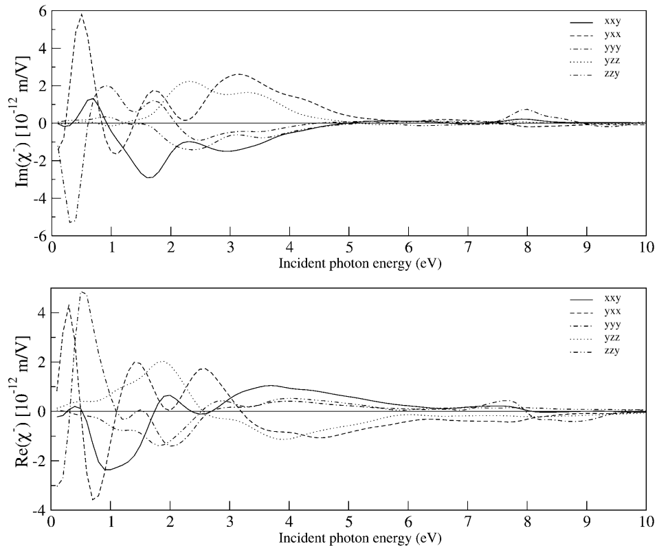
FIGURE 2 Spectral dependence of the odd (in magnetization) components of the \chi_{ijk} tensor for the Ni/Cu(001) bilayer with the in-plane magnetization direction
