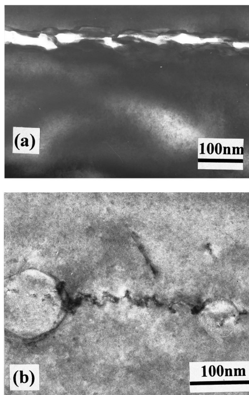
FIG. 5. XTEM image of the 4.5 \times 10^{16} atoms/cm 2 , 140 kV H + -implanted Si after annealing at 1000 °C for 2 h, showing (a) crack at the projected range; (b) cavity with a string of interconnected platelets.
