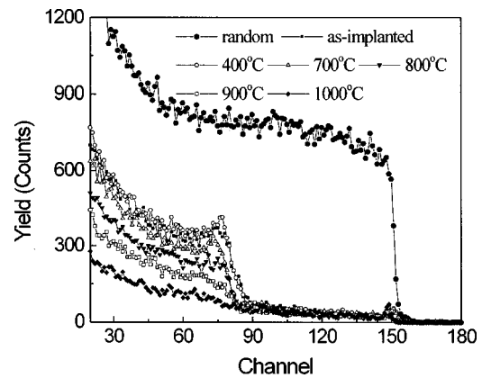
FIG. 1. Channeling RBS spectra of the Si sample implanted with 3 \times 10^{16} atoms/cm 2 , 140 kV \text{H}^+ and annealed at different temperature for 30 min.
