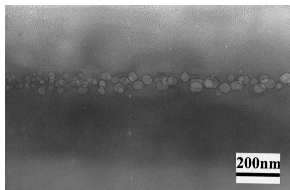
FIG. 4. XTEM image of the 4.5 \times 10^{16} atoms/cm 2 , 140 kV H + -implanted Si after annealing at 900 °C for 2 h showing more microcavities than the sample shown in Fig. 2.
