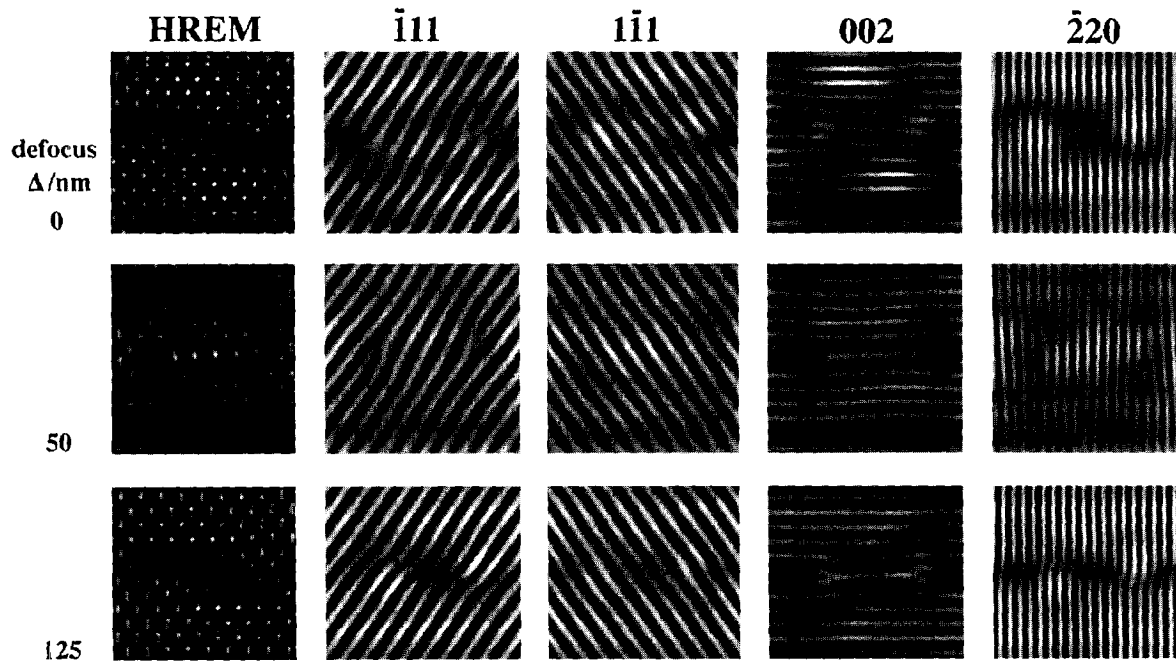
Fig. 5. MD simulated (001)-Si wafer bonding at double steps: theoretical 200 kV-[110]-HREM and filtered images (spherical aberration = 1 mm, defocus spread = 1 nm, beam divergence = 0.05 mrad, thickness = 7.9 nm).
