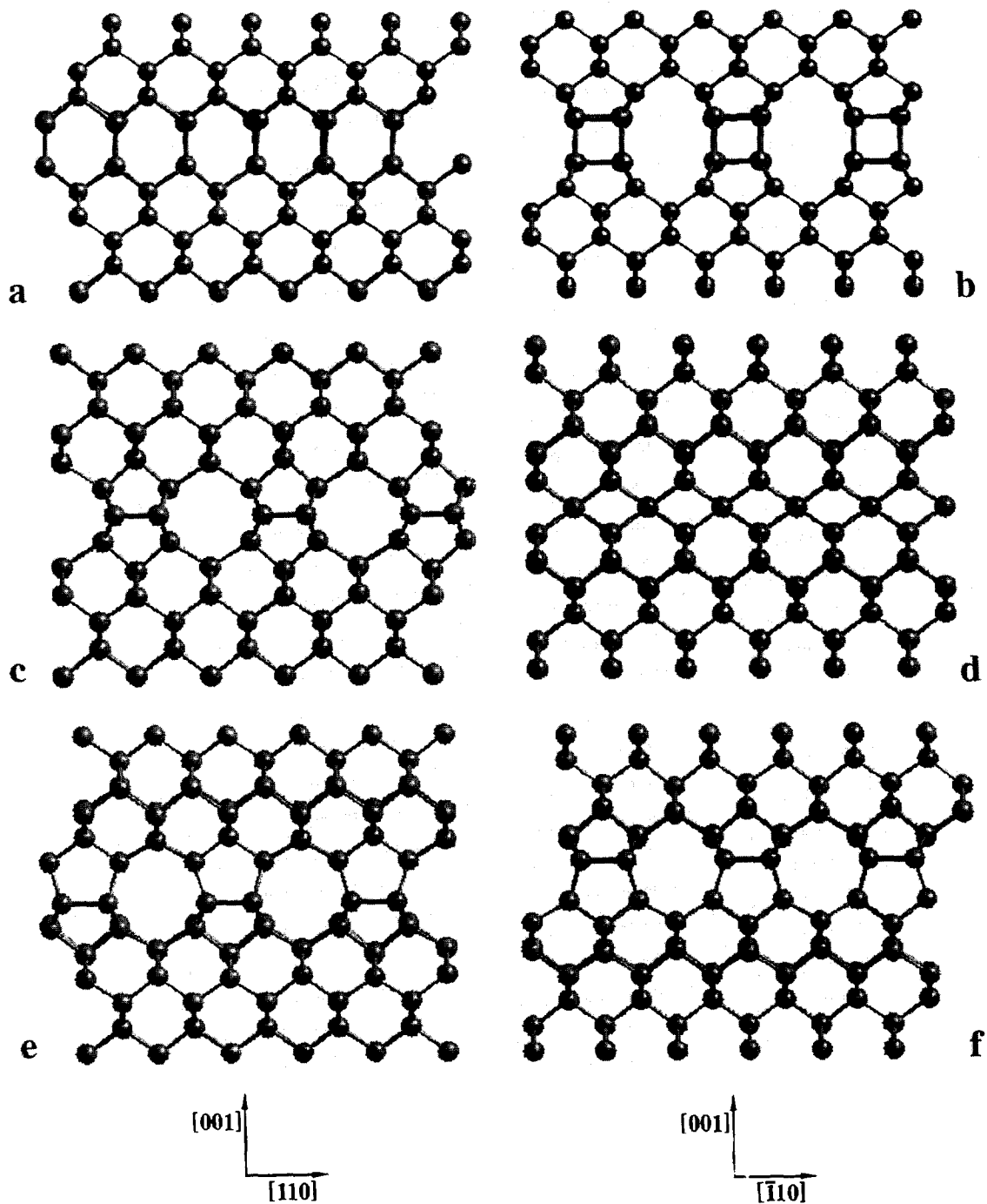
Fig. 1. MD relaxed interface structures of bonded Si(001) interfaces, [\bar{1}10] and [110] projections: (a, b) parallel dimers, fast heat, Stillinger–Weber, (c, d) orthogonal dimers, slow heat, Stillinger–Weber, (e, f) dito with Tersoff.
