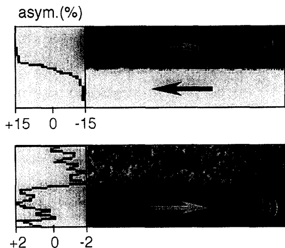
Fig. 2. (a) Magnetic domain pattern of a clean Fe(100) whisker surface recorded with Fe LMV Auger electrons. The image shows a region with a single 180^\circ wall (inset: vertical line scan showing the contrast between the two oppositely magnetized domains). (b) Magnetic domain pattern in a chromium monolayer deposited onto the iron surface in (a). This image was obtained with Cr LMV Auger electrons ( E_{kin} = 529 eV) and excitation at the Cr L_{2,3} edge (inset: vertical line scan showing the contrast reversal due to the antiferromagnetic coupling of the Cr overlayer to the Fe substrate).
