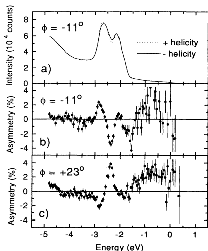
FIG. 2. (a) The angle-resolved photoemission intensity spectra from Cu(001) using a photon energy of 12 eV and emission angles of \theta = 23^\circ and \phi = -11^\circ plotted against the initial-state energy. Light of positive (dotted line) and negative (solid line) helicity was used. (b) The intensity asymmetry for the spectra in part (a). (c) The intensity asymmetry for a different emission angle \phi = +23^\circ .
