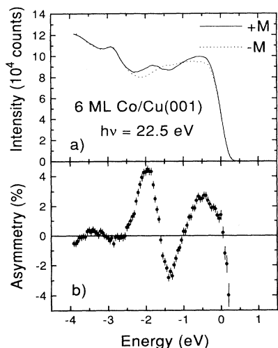
FIG. 1. (a) Angle-resolved photoemission intensity spectra from a 6-ML Co film on a Cu(001) substrate for remanent magnetization in the surface plane along [110] ( +M ) and [-1-10] ( -M ). The experimental geometry is given in the text. (b) The intensity asymmetry for the spectra in (a).
