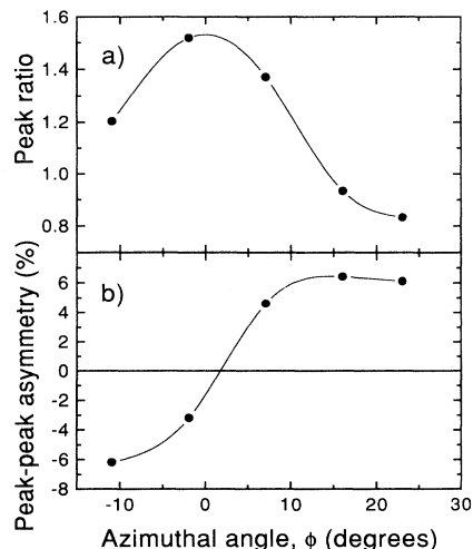
FIG. 3. (a) The ratio of the heights of the two peaks seen in the photoemission spectra in Fig. 2(a) as a function of the azimuthal angle of emission, \phi . (b) The peak-to-peak size of the \pm feature in the intensity asymmetry as a function of \phi .
