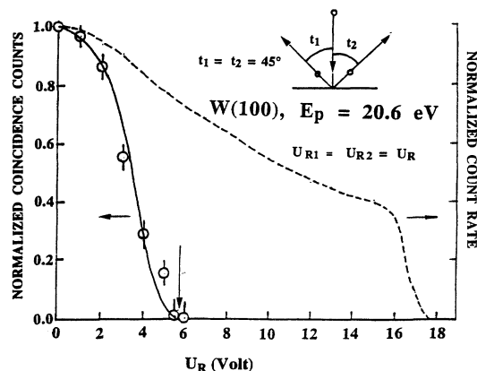
FIG. 4. Number of true coincidence events as a function of retarding potential applied to detector grids. Angle of incidence \Theta = 0^\circ , detection angles t_1 = 45^\circ , t_2 = -45^\circ , retarding potentials U_{R1} = U_{R2} = U_R . The arrow indicates the energy-conservation-law limit ( U_R = 5.7 V). Parameters of calculation are the same as in Fig. 2. The right-hand scale is the secondary-electron rate (dashed curve).
