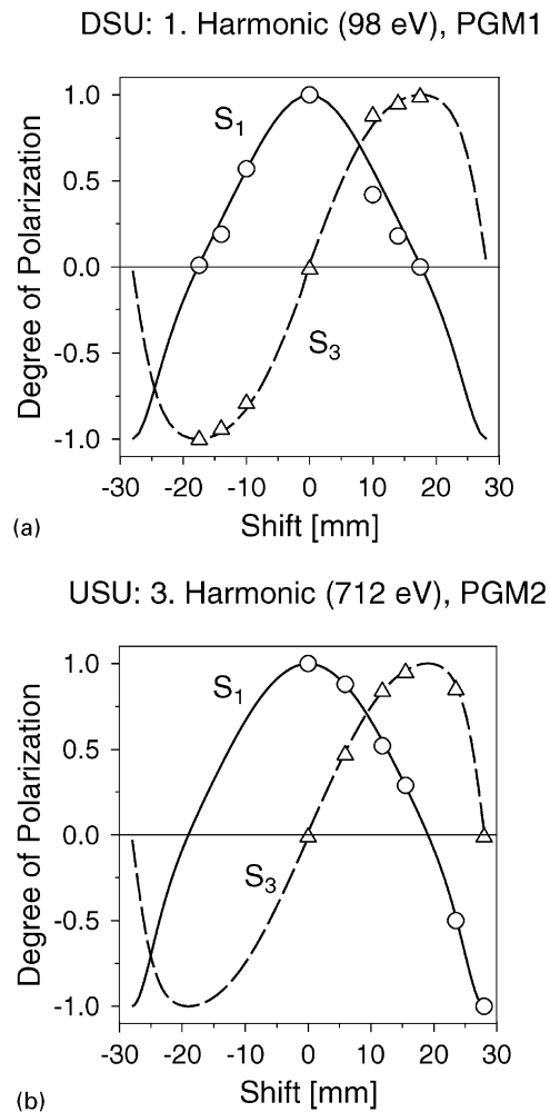
Fig. 3. Degree of circular polarization S_3 and linear polarization S_1 as a function of undulator's longitudinal shift for 98 eV (a) in first undulator harmonic, and for 712 eV (b) in the third harmonic. Symbols: measured values; lines: calculations.
