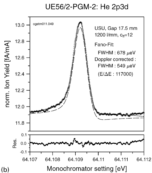
Fig. 2. (a) Autoionization spectrum of doubly excited helium. The principle series was resolved up to the 35 resonance. The inset shows the very sharp 2p3d feature. (b) Detailed measurement of the 2p3d peak, showing a Doppler-broadened FWHM of 690 \mu\text{eV} .
