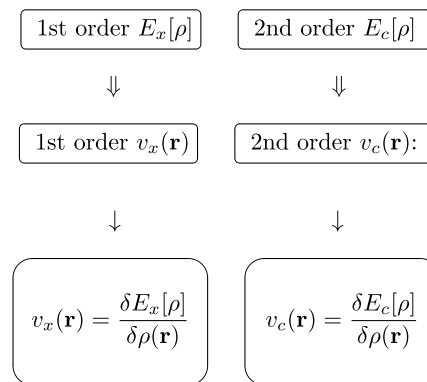
Fig. 1. Traditional DFT PT scheme linking the exchange energy E_x[\rho] with the exchange potential v_x(\mathbf{r}) in first order, and the correlation energy E_c[\rho] with the correlation potential v_c(\mathbf{r}) in second order.
