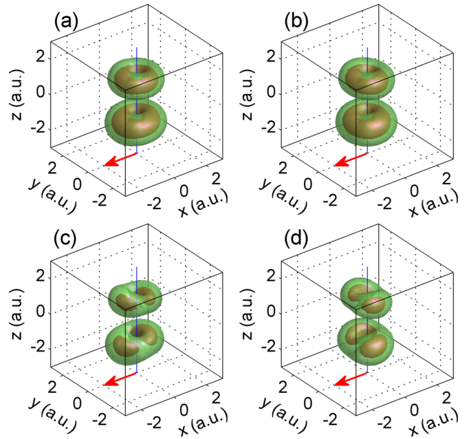
FIG. 3. Snapshots of the electron probability densities at t = 1.5 T for the initial 2\pi_+ (left column) and 2\pi_- (right column) orbitals. The arrows indicate the direction of the instantaneous electric field vector. The wavelength of the three-cycle laser pulse is \lambda = 1600 nm and the electric field amplitudes are \mathcal{E} = 0.05 a.u. (top row) and 0.11 a.u. (bottom row).
