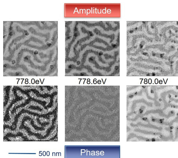
Figure 11. Reconstructed soft x-ray ptychography magnetic amplitude (top row) and phase (bottom row) images of the domain pattern in a SmCo 5 thin film recorded with left circularly polarized x-rays at various photon energies around the Co L 3 absorption edge. Reprinted from [78], with the permission of AIP Publishing.
