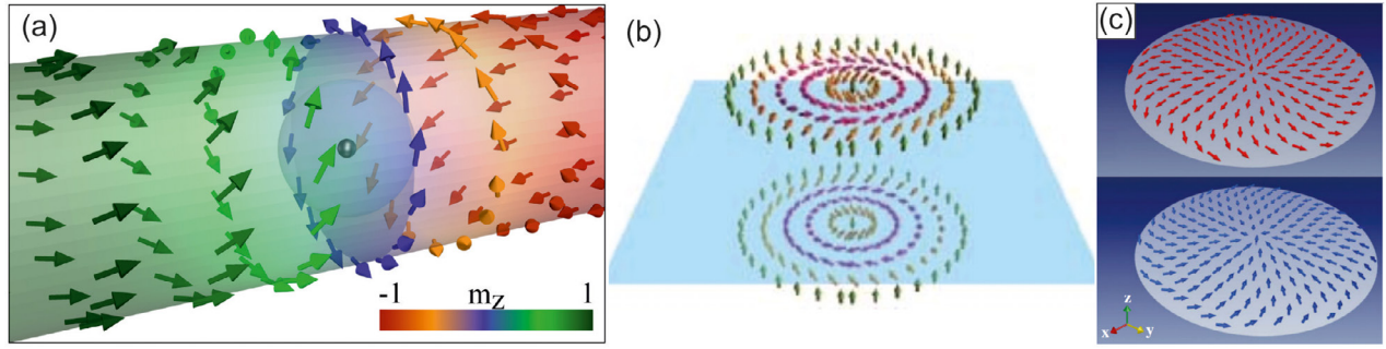
Figure 6. Topologically non-trivial spin textures. (a) A vortex domain wall in a solid cylindrical ferromagnetic wire contains a Bloch point, at which the magnetisation direction cannot be defined. Reproduced from [50]. © IOP Publishing Ltd. All rights reserved. (b) A Bloch skyrmion and its mirror image, on to which it cannot be superimposed. It is thus a chiral object. Reproduced from [52]. © 2015 Chinese Physical Society and IOP Publishing Ltd. All rights reserved. (c) Spin structure of a meron-like state with opposite chiralities in a pair of coupled magnetic discs. Adapted with permission from [58]. Copyrighted by the American Physical Society.
