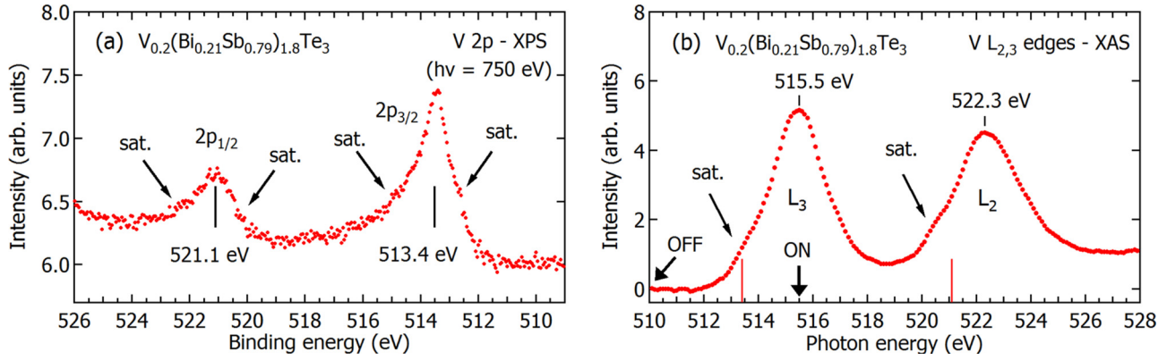
FIG. 1. Representative spectra of (a) the V 2p core levels, measured at h\nu = 750 eV, and (b) the V L_{2,3} edges from a V_{0.2}(Bi_{0.21}Sb_{0.79})_{1.8}Te_3 (4 at.%) film. Satellite structures (labeled “sat.”) characterize the V 2p and L -edge lineshapes in this system. The red lines mark the position of the V 2p core levels. The L_3 -edge maximum is found 1.9 eV above the 2p_{3/2} peak. The labels ON and OFF mark the photon energies used in the resPES measurements.
