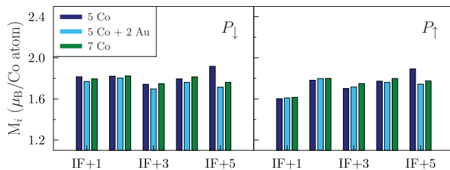
FIG. 8. (Color online) Distribution of magnetic moments in a Co film along [001] calculated for the two polarizations, P_{\downarrow} (left panel) and P_{\uparrow} (right panel), of the PTO substrate. Results for three Co films (see Fig. 1) are shown.
