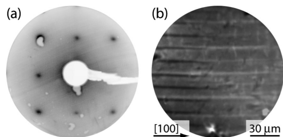
FIG. 1. (a) LEED and (b) PEEM of the BTO(001) surface after UHV preparation [(a) E = 60 eV, T = 300 K; (b) FOV = 150 \mu\text{m} , h\nu = 4.35 eV, approximately 330 K]. The sample reveals a stripelike domain pattern consisting of all three domain types, discriminable by their different photoemission yields.
