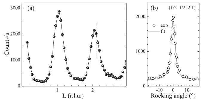
FIG. 8. (a) L scan along the (1/2 1/2)-rod for the MnPt film deposited at RT and annealed at 770 K. The vertical (dash) line indicates the position for the rocking scan shown in (b).
