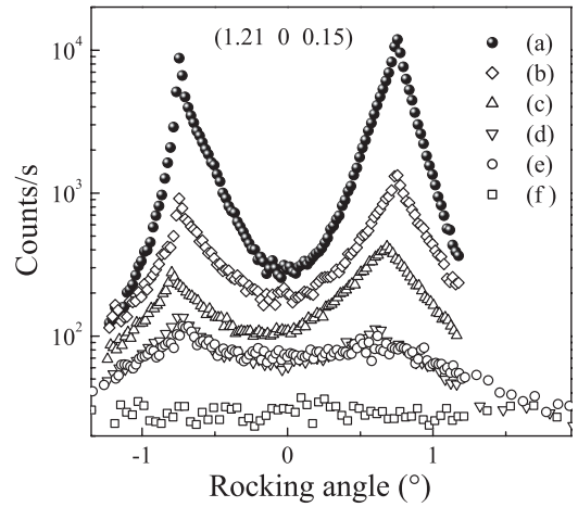
FIG. 2. Rocking scans around the (1.21 \ 0 \ 0.15) reciprocal space point of the Pt(001)-hex reconstruction rod for selected surfaces: (a) freshly clean surface; (b) immediately after 0.35-ML Mn deposition (19%); (c) 0.35-ML Mn after 10 hours (8%); (d) 0.35-ML Mn after 30 min annealing at 520 K (3%); (e) 1.2-ML Mn deposition on a freshly clean surface (2%); and (f) 1.2-ML Mn + 1-ML Pt (0%). The number in parenthesis is the remaining percentage of Pt(001)-hex reconstruction relative to the freshly clean surface.
