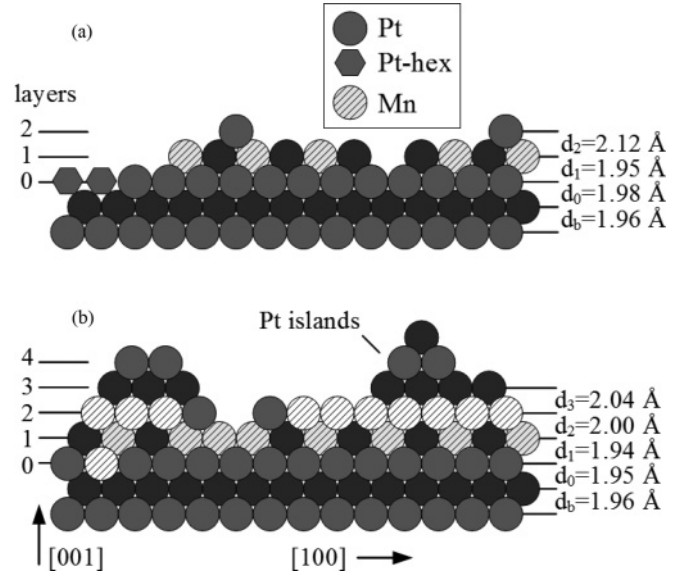
FIG. 4. Sketch of the model structure for the (a) 0.35-ML Mn and (b) 1-ML Pt/1.2-ML Mn, deposited at RT on Pt(001)-hex. The distances obtained by fit are given. The sketch (a) shows some remaining reconstruction, but no Mn atoms, in layer 0, and a MnPt- c(2 \times 2) surface alloy in an incomplete layer 1. (b) shows the same ordered alloy with the layer 1 completed by Mn atoms, the excess of Mn covering partially the layer 2 and the 3D growth of islands after Pt deposition.
