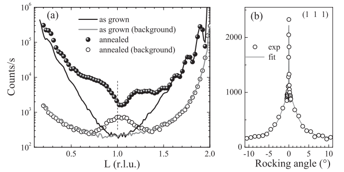
FIG. 7. (a) L scans along the (1 1)-CTR for the (MnPt) 6 film as deposited at RT (black solid line) and after annealing at 770 K (full circles). The offset scans, along (1.03 1.03), before annealing (gray solid line) give the background, and after annealing, show a broad peak coming from L1_0 domains. The vertical (dash) line indicates the position for the rocking scan shown in (b).
