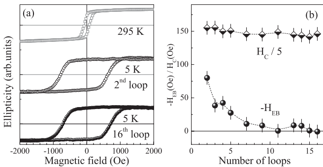
FIG. 12. (a) Polar MOKE hysteresis loops of the Pt/FePt/MnPt HT film at 295 K (squares) and after perpendicular magnetic field cooling ( H_{\text{MFC}} = 3000 Oe) down to 5 K: (open circles) second loop and (closed circles) sixteenth loop. (b) Coercivity ( H_C ) and exchange bias shift ( -H_{\text{EB}} ) as a function of the number of loops measured. (Lines are guides to the eye.)
