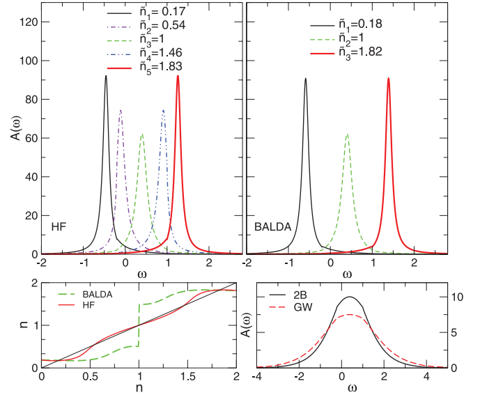
FIG. 2. (Color online) Spectral functions for the different steady-state solutions of the HF approximation (top-left panel) and BALDA (top-right panel). The graphical solution of Eq. (15) is displayed in the bottom-left panel for the HF and BALDA. For comparison we also report the 2B and GW steady-state spectral functions in the bottom-right panel.
