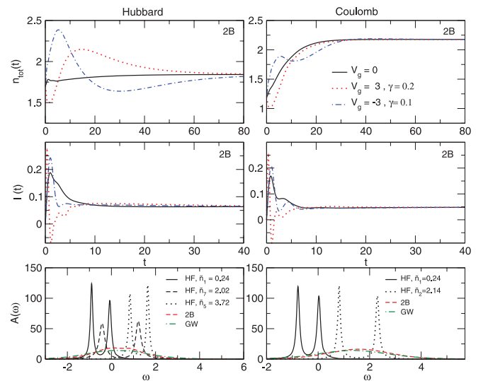
FIG. 10. (Color online) Densities and currents for the 2B approximation short-range (Hubbard) and long-range (Coulomb) interactions are used. Lower panel: Spectral functions for the different approximations at the end of the time propagation.
