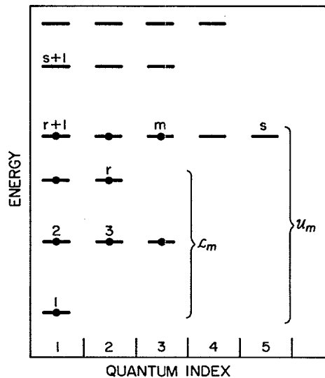
FIG. 1. The spectrum of the Hamiltonian H , Eq. (1), depicted schematically. The horizontal axis represents an index distinguishing between degenerate levels (e.g., the magnetic quantum number of orbitally degenerate atomic states). The vertical axis displays the energy. The solid circles identify the levels in the ensemble of the first m eigenstates. The curly brackets indicate the sets \mathcal{L}_m \equiv [|\phi_1\rangle, |\phi_2\rangle, \dots, |\phi_m\rangle] and \mathcal{U}_m \equiv [|\phi_1\rangle, |\phi_2\rangle, \dots, |\phi_m\rangle] . As the relation (6) suggests, the m th state in the spectrum is generally degenerate, and in general the highest multiplet (i.e., the multiplet |r+1\rangle, |r+2\rangle, \dots, |m\rangle, \dots, |s\rangle ) in that ensemble is partially occupied.
