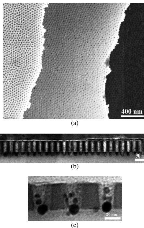
Figure 2. Electron microscopy images of nanoporous \text{Si}_3\text{N}_4 -coated Si wafers after the dry plasma etching step, but prior to the thermal treatment. (a) SEM image showing the Au-coated porous PS film (on the left), the intermediate \text{Si}_3\text{N}_4 layer (in the middle), and the underlying Si wafer (on the right). ((b), (c)) TEM images of cross-sectional specimens of nanoporous arrays cut parallel to the long axes of the pores prior to and after the deposition of Au, respectively.
