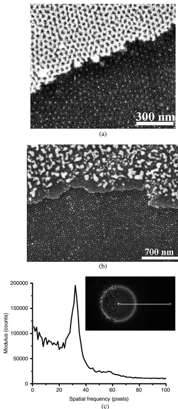
Figure 3. SEM images of wafers after dry plasma etching and decoration with Au. Au-coated porous PS films (at the top) and Au nanoparticles within the pores of ordered nanoporous Si (at the bottom) (a) prior to the thermal treatment and (b) after annealing at 450 °C for 30 min. (c) Modulus profile of the averaged Fourier transform (inset, right) obtained from a square section of the lower part of figure 3(b). The modulus profile was taken along the line indicated in the inset (zero-coefficient out of plotted range).
