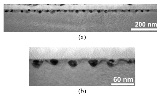
Figure 4. TEM images of cross-sectional specimens cut normal to the sample surface of nanoporous Si wafers, which were decorated with Au nanoparticles and then annealed at 600 °C for 30 min. (a) Overview; (b) detail.
