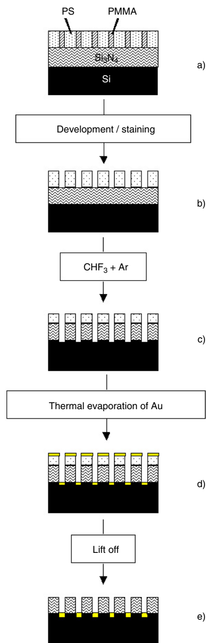
Figure 1. Schematic diagram of the fabrication procedure for high-temperature resistant Au nanoparticle arrays. (a) A film consisting of asymmetric PS- b -PMMA containing PMMA cylinders oriented normal to the film plane is formed on a Si wafer coated with Si 3 N 4 and P(S- r -MMA). (b) An ordered porous PS film obtained by selective removal of the PMMA is stained with RuO 4 . (c) The pore pattern is transferred into the wafer by dry plasma etching with a CHF 3 /Ar mixture. (d) The sample is decorated with Au by thermal evaporation in high vacuum. (e) The polymer layer and the residual Au on the surface are lifted off.
