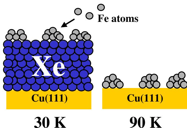
Figure 19. A schematic picture depicting the various steps of the buffer-layer-assisted growth process.
